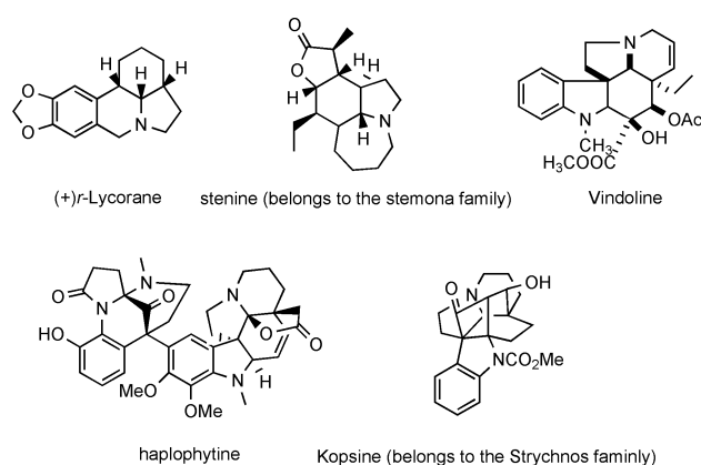
Scheme 1. Several natural products that contain the fragments of 5-substituted 3-pyrrolidin-2-one derivatives.
