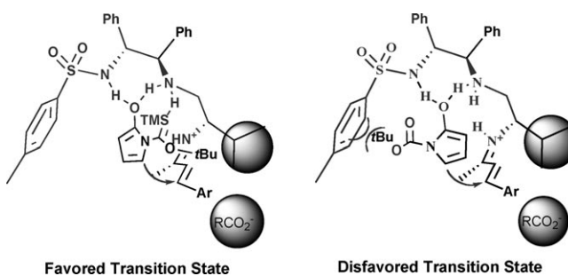
Scheme 2. Proposed transition state in the vinylogous Michael reaction.
