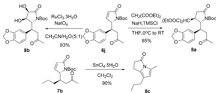
Scheme 3. Several examples of the transformations of the corresponding Michael products. THF = tetrahydrofuran, TMS = trimethylsilyl.
